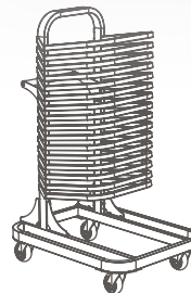
ROUND / SQUARE TOP TRANSFER AND STORAGE CART L40" W31" H61" L101cm W79cm H155cm holds up to 16 PoLo round/square tops MG CUUX04 XXXX
